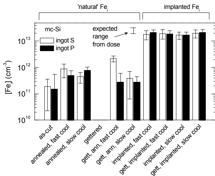
Figure 3. Fe_i concentrations in the multicrystalline samples for the 2 ingots. For the implanted samples (at right) the expected Fe_i concentration is the dose divided by the wafer thickness.
