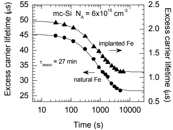
Figure 2. Decrease in carrier lifetime (at \Delta n = 5 \times 10^{15} \text{ cm}^{-3} ) as the FeB pairs re-form after illumination ( T = 31^\circ\text{C} ). An exponential fit (solid line) gave an identical re-pairing time \tau_{\text{assoc}} of 27 minutes for mc-Si samples containing implanted or 'natural' Fe_i .
