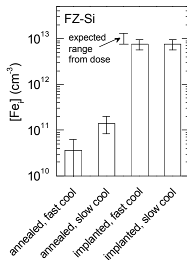
Figure 4. Fe_i concentrations in the FZ samples.
