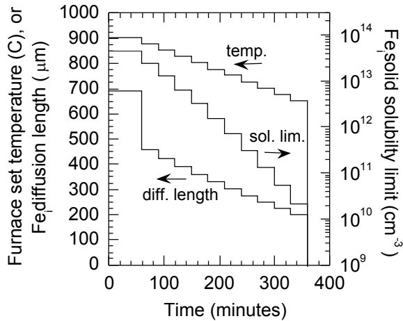
Figure 1. Temperature profile for the slow-cooled samples. Also shown are the solid solubility limits and the diffusion lengths for Fe_i at each temperature step.
