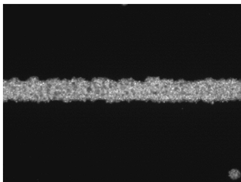
Figure 1.. Image of inkjet seed & Cu plate finger of the front grid.
