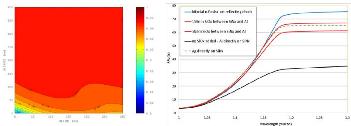
Figure 6.. a (Left): Calculated internal rear reflectance for a layer of SiO x (vertical axis = SiO x thickness) between SiN x (horizontal axis = SiN x thickness) and Aluminium. b (Right): experimental result for escape reflection for different rear side stacks. The red curves (SiO x added) compared to the black curve (no SiO x added, situation of Table 3 and Fig. 3) show how
