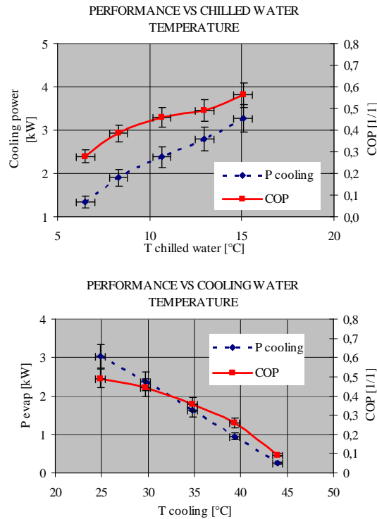
Figure 4: Influence of cooling water (below) and chilled water (upper) inlet temperature
